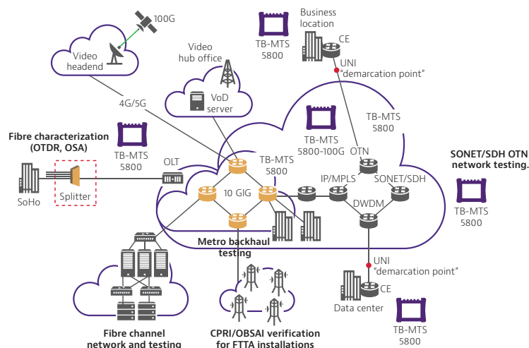
Figure 1. T-BERD/MTS-5800 in the carrier Ethernet network
